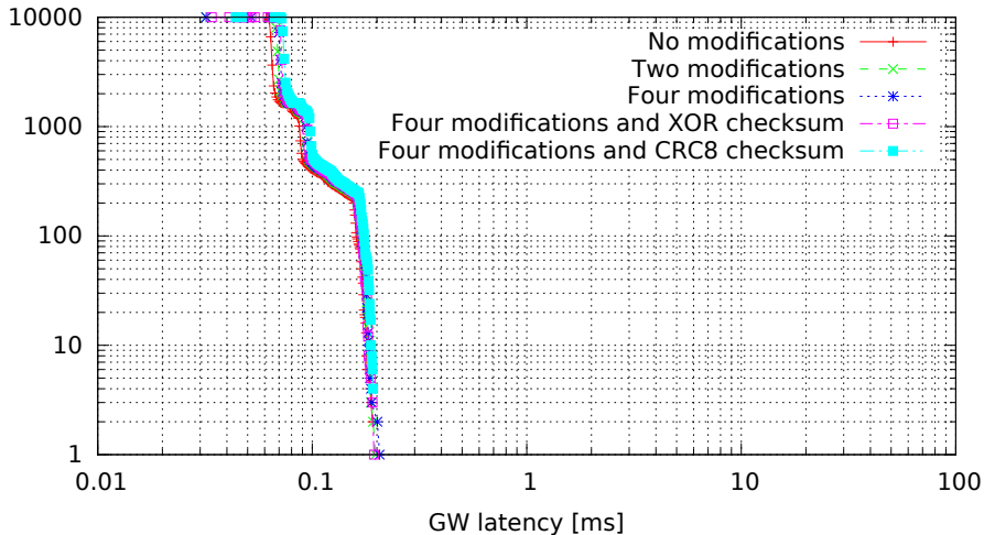
Single GW rule for all messages with modifications, 8 byte messages (GW kernel 3.0.4-rt14-00008-gb2052fd, Traffic 50, Load none)
