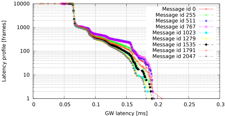
2048 GW rules (one per id, mask C00007FF), no modifications (GW kernel 3.0.4-rt14-00008-gb2052fd, Traffic 50, Load none)
