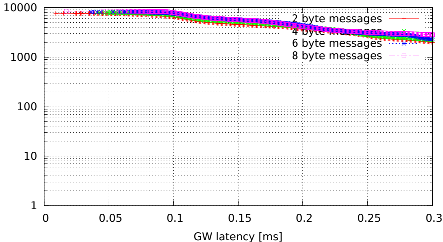
Single GW rule for all messages, no modifications (GW kernel 3.0.4-rt14-00008-gb2052fd, Traffic 50, Load eth)
