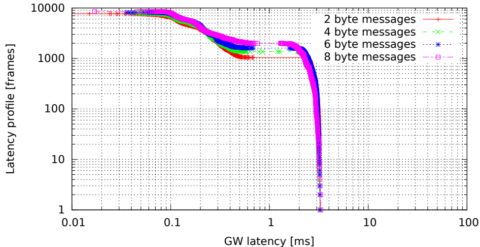
Single GW rule for all messages, no modifications (GW kernel 3.0.4-rt14-00008-gb2052fd, Traffic 50, Load eth)
