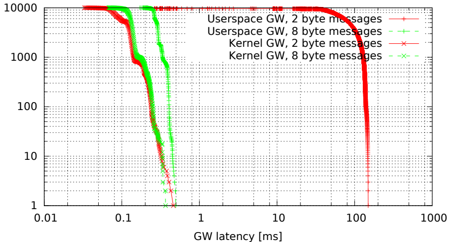
Kernel vs. userspace GW, no modifications (GW kernel 3.0.4-rt14-00008-gb2052fd, Traffic 50, Load cpu)
