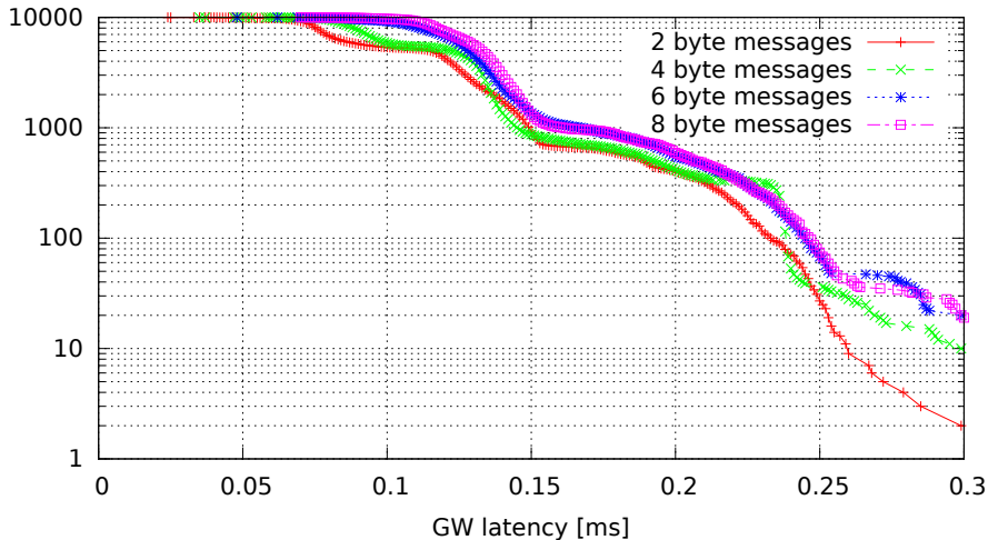
Single GW rule for all messages, no modifications (GW kernel 3.0.4-rt14-00008-gb2052fd, Traffic 50, Load cpu)
