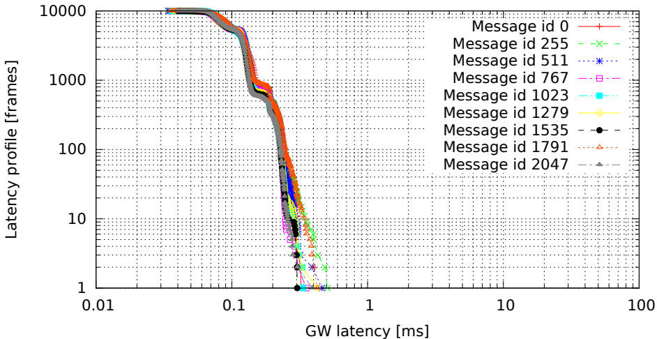
2048 GW rules (one per id, mask C00007FF), no modifications (GW kernel 3.0.4-rt14-00008-gb2052fd, Traffic 50, Load cpu)
