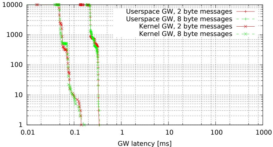
Kernel vs. userspace GW, no modifications (GW kernel 3.0.4-00007-g1c8c373, Traffic oneatatime, Load none)
