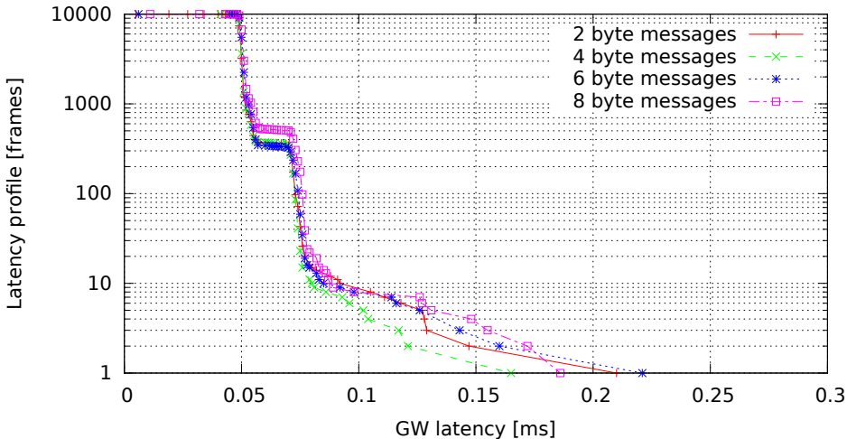
Single GW rule for all messages, no modifications, high (soft)irq task priority (GW kernel 3.0.4-00007-g1c8c373, Traffic oneatatime, Load none)
