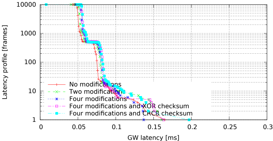
Single GW rule for all messages with modifications, 8 byte messages (GW kernel 3.0.4-00007-g1c8c373, Traffic oneatatime, Load none)
