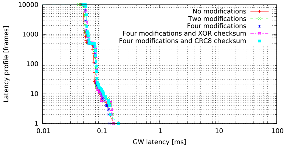
Single GW rule for all messages with modifications, 8 byte messages (GW kernel 3.0.4-00007-g1c8c373, Traffic onetatime, Load none)
