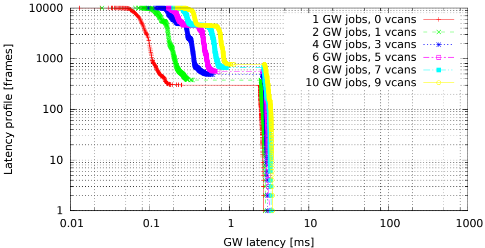
Chained GWs on multiple VCAN interfaces (GW kernel 3.0.4-00007-g1c8c373, Traffic oneatatime, Load eth)
