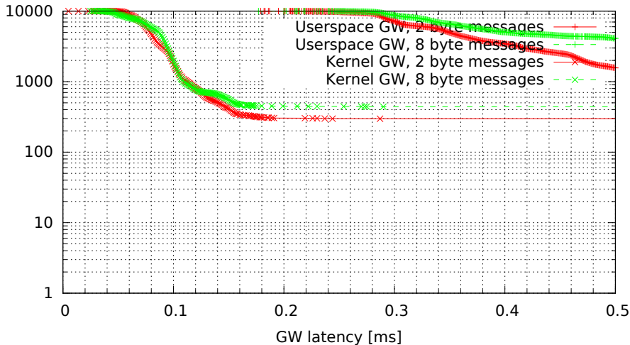
Kernel vs. userspace GW, no modifications (GW kernel 3.0.4-00007-g1c8c373, Traffic oneatatime, Load eth)
