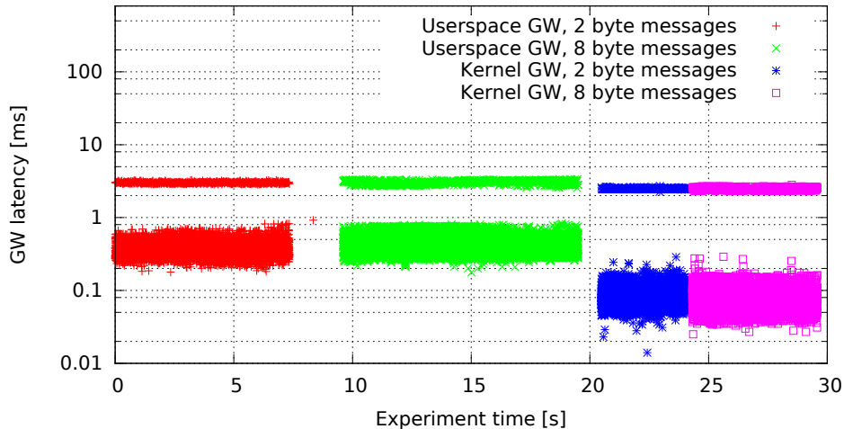
Single GW rule for all messages, no modifications (GW kernel 3.0.4-00007-g1c8c373, Traffic oneatatime, Load eth)
