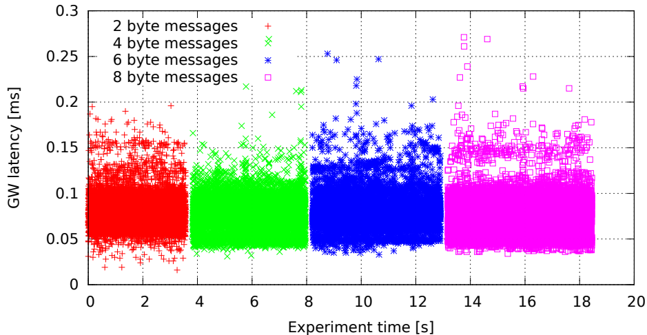
Single GW rule for all messages, no modifications, high (soft)irq task priority (GW kernel 3.0.4-00007-g1c8c373, Traffic oneatatime, Load eth)
