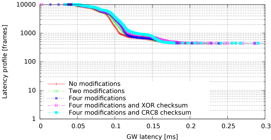
Single GW rule for all messages with modifications, 8 byte messages (GW kernel 3.0.4-00007-g1c8c373, Traffic oneatatime, Load eth)
