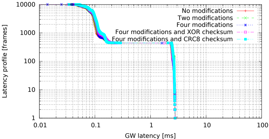
Single GW rule for all messages with modifications, 8 byte messages (GW kernel 3.0.4-00007-g1c8c373, Traffic onetatime, Load eth)
