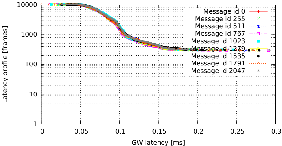
2048 GW rules (one per id, mask C00007FF), no modifications (GW kernel 3.0.4-00007-g1c8c373, Traffic oneatatime, Load eth)
