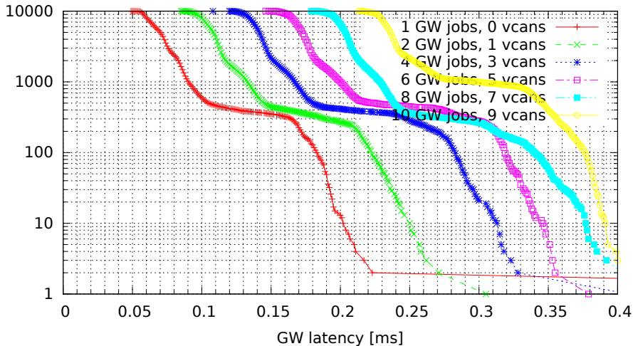
Chained GWs on multiple VCAN interfaces (GW kernel 3.0.4-00007-g1c8c373, Traffic onetatime, Load cpu)
