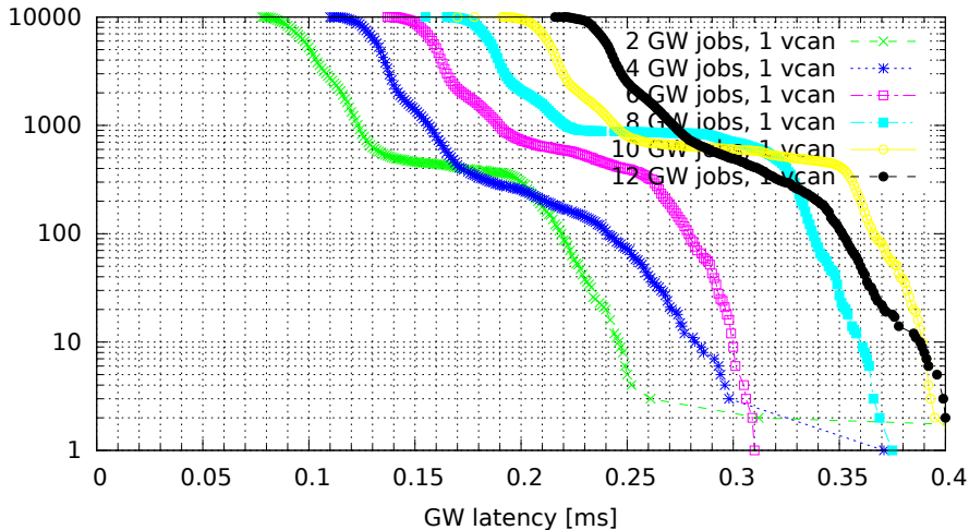
Chained GWs on a single VCAN interface (GW kernel 3.0.4-00007-g1c8c373, Traffic onetatime, Load cpu)
