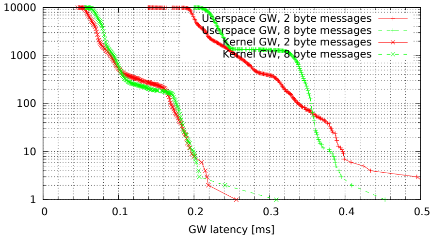
Kernel vs. userspace GW, no modifications (GW kernel 3.0.4-00007-g1c8c373, Traffic oneatatime, Load cpu)
