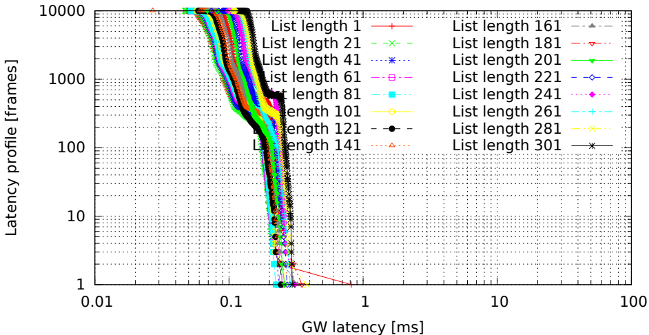
Different lengths of filter list, only the last one matches (GW kernel 3.0.4-00007-g1c8c373, Traffic oneatatime, Load cpu)
