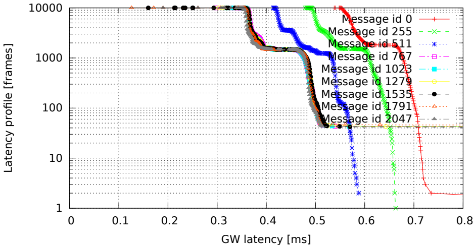
2048 GW rules (one per id, mask 0x7FF), no modifications (GW kernel 3.0.4-00007-g1c8c373, Traffic oneatatime, Load cpu)
