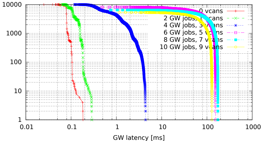
Chained GWs on multiple VCAN interfaces (GW kernel 3.0.4-00007-g1c8c373, Traffic flood, Load none)
