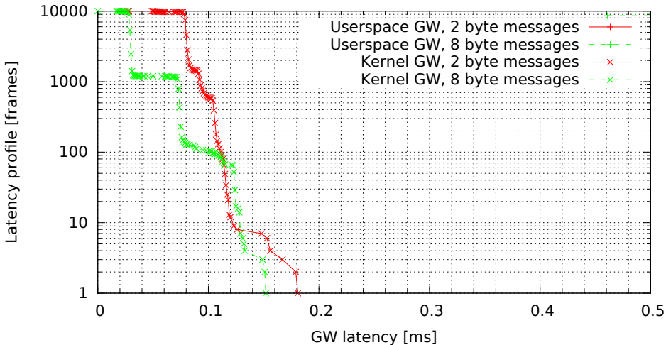
Kernel vs. userspace GW, no modifications (GW kernel 3.0.4-00007-g1c8c373, Traffic flood, Load none)
