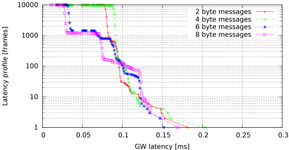
Single GW rule for all messages, no modifications, high (soft)irq task priority (GW kernel 3.0.4-00007-g1c8c373, Traffic flood, Load none)
