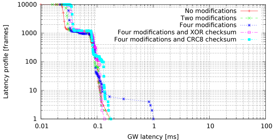
Single GW rule for all messages with modifications, 8 byte messages (GW kernel 3.0.4-00007-g1c8c373, Traffic flood, Load none)
