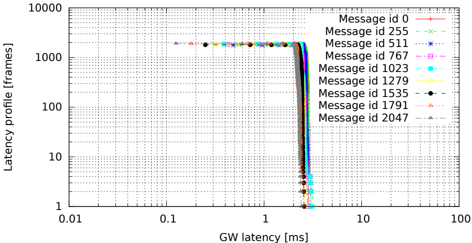
2048 GW rules (one per id, mask 0x7FF), no modifications (GW kernel 3.0.4-00007-g1c8c373, Traffic flood, Load none)
