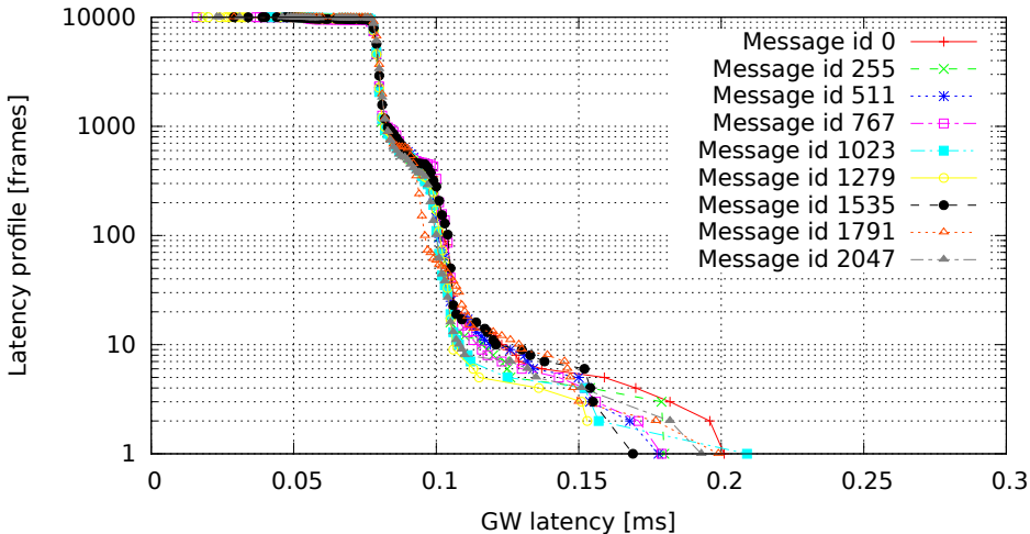
2048 GW rules (one per id, mask C00007FF), no modifications (GW kernel 3.0.4-00007-g1c8c373, Traffic flood, Load none)
