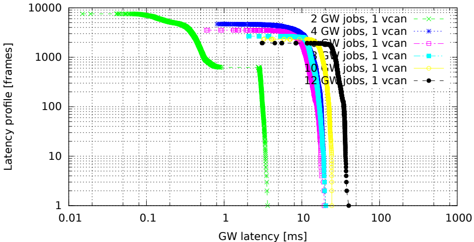
Chained GWs on a single VCAN interface (GW kernel 3.0.4-00007-g1c8c373, Traffic flood, Load eth)
