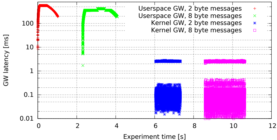
Single GW rule for all messages, no modifications (GW kernel 3.0.4-00007-g1c8c373, Traffic flood, Load eth)
