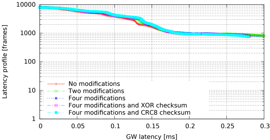
Single GW rule for all messages with modifications, 8 byte messages (GW kernel 3.0.4-00007-g1c8c373, Traffic flood, Load eth)
