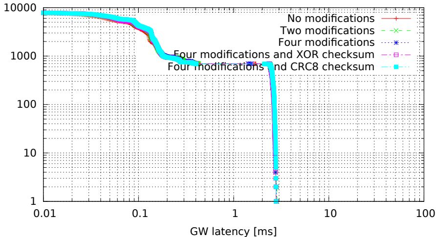
Single GW rule for all messages with modifications, 8 byte messages (GW kernel 3.0.4-00007-g1c8c373, Traffic flood, Load eth)
