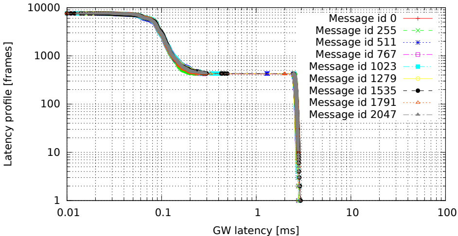
2048 GW rules (one per id, mask C00007FF), no modifications (GW kernel 3.0.4-00007-g1c8c373, Traffic flood, Load eth)
