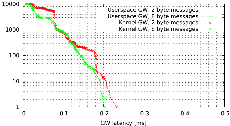
Kernel vs. userspace GW, no modifications (GW kernel 3.0.4-00007-g1c8c373, Traffic flood, Load cpu)
