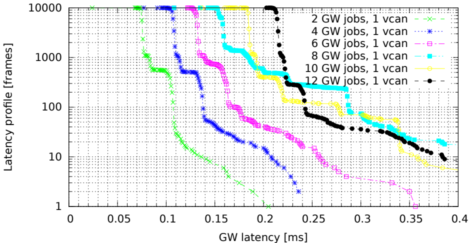
Chained GWs on a single VCAN interface (GW kernel 3.0.4-00007-g1c8c373, Traffic 50, Load none)
