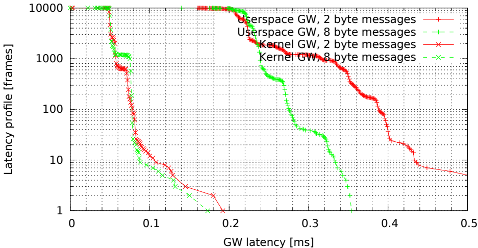
Kernel vs. userspace GW, no modifications (GW kernel 3.0.4-00007-g1c8c373, Traffic 50, Load none)
