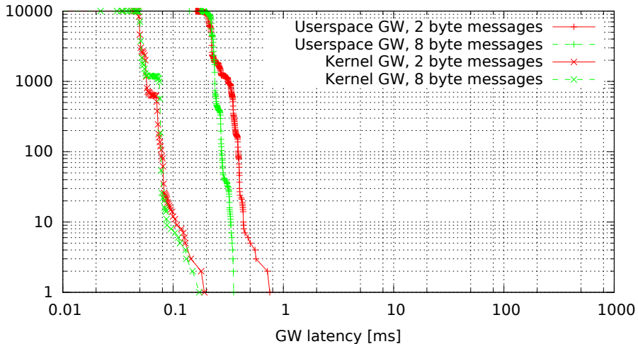
Kernel vs. userspace GW, no modifications (GW kernel 3.0.4-00007-g1c8c373, Traffic 50, Load none)
