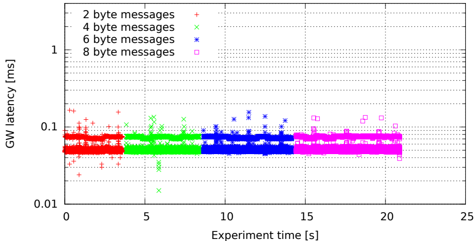
Single GW rule for all messages, no modifications, high (soft)irq task priority (GW kernel 3.0.4-00007-g1c8c373, Traffic 50, Load none)
