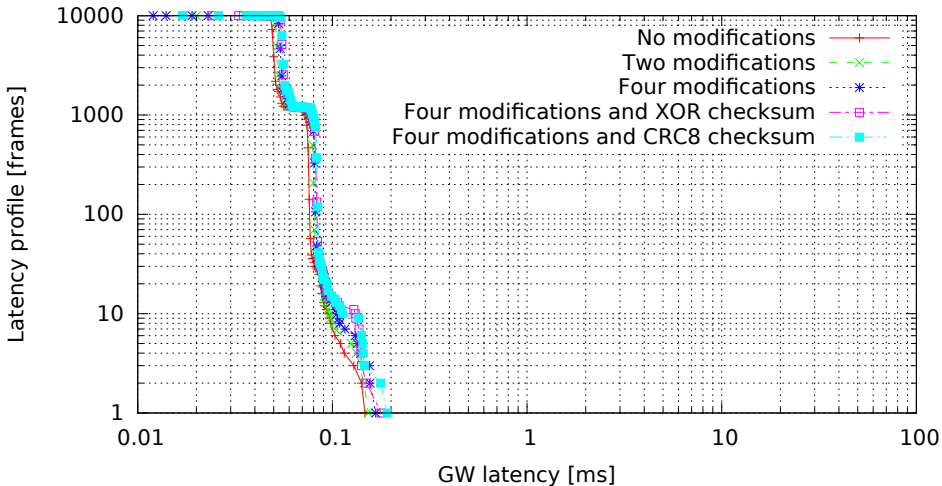
Single GW rule for all messages with modifications, 8 byte messages (GW kernel 3.0.4-00007-g1c8c373, Traffic 50, Load none)
