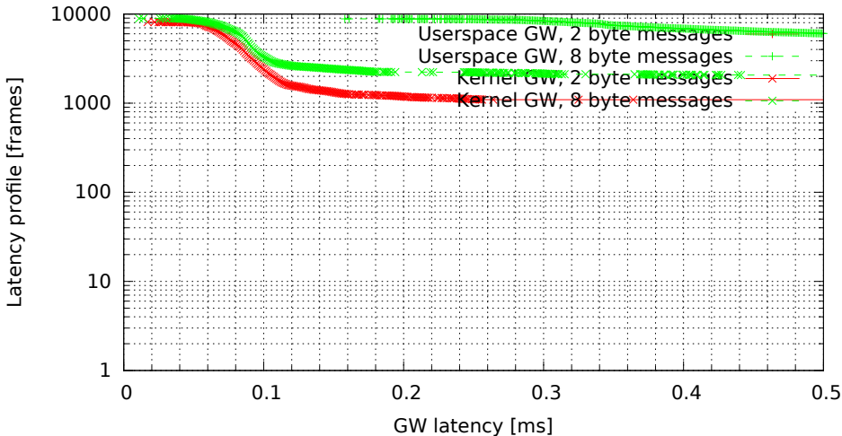
Kernel vs. userspace GW, no modifications (GW kernel 3.0.4-00007-g1c8c373, Traffic 50, Load eth)
