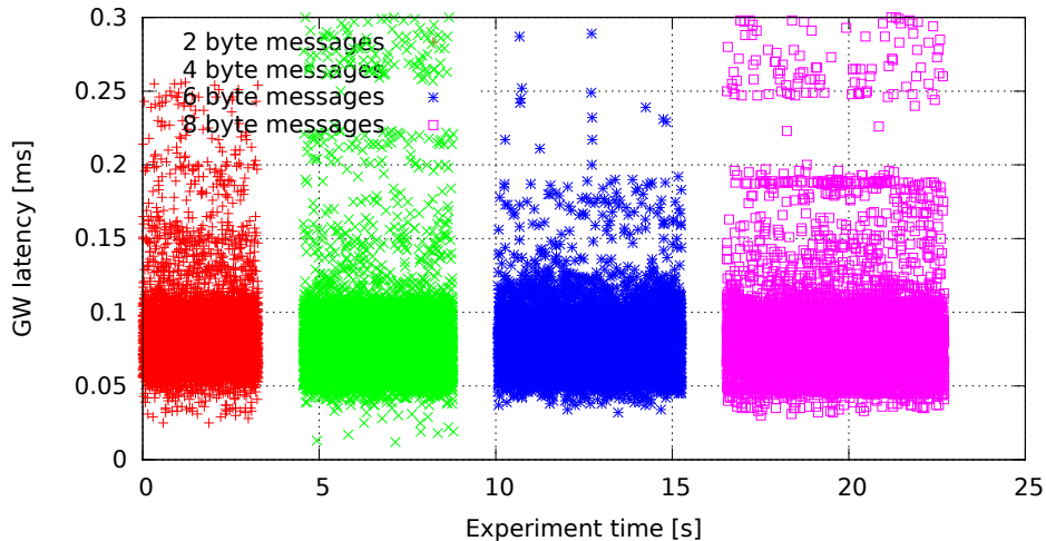
Single GW rule for all messages, no modifications (GW kernel 3.0.4-00007-g1c8c373, Traffic 50, Load eth)
