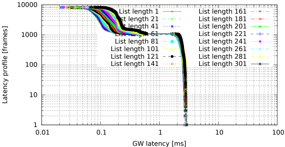
Different lengths of filter list, only the last one matches (GW kernel 3.0.4-00007-g1c8c373, Traffic 50, Load eth)
