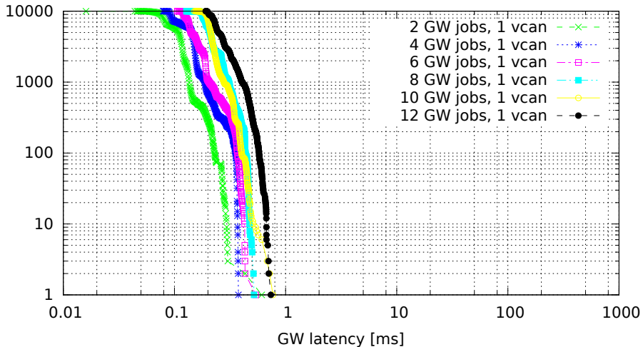
Chained GWs on a single VCAN interface (GW kernel 3.0.4-00007-g1c8c373, Traffic 50, Load cpu)
