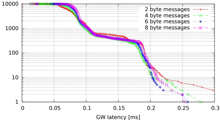
Single GW rule for all messages, no modifications (GW kernel 3.0.4-00007-g1c8c373, Traffic 50, Load cpu)
