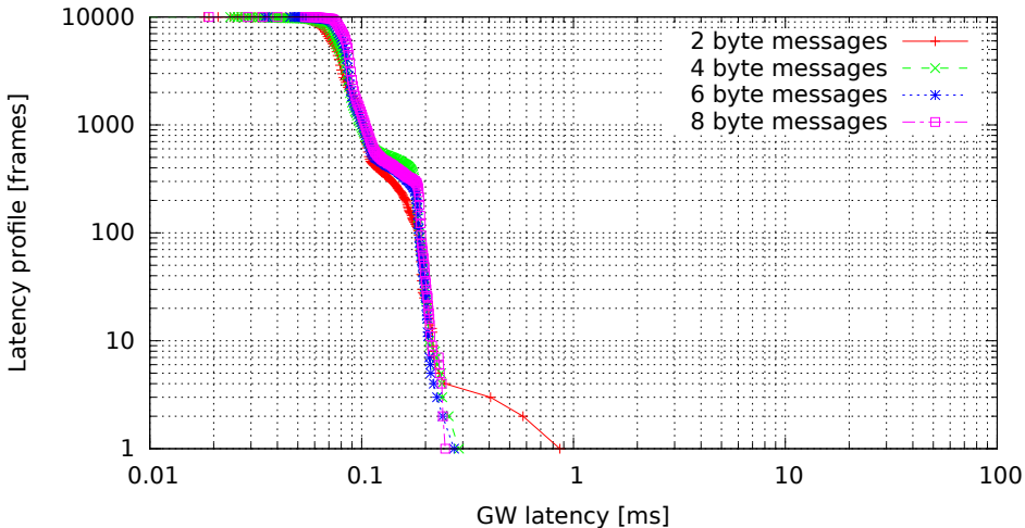
Single GW rule for all messages, no modifications, high (soft)irq task priority (GW kernel 3.0.4-00007-g1c8c373, Traffic 50, Load cpu)
