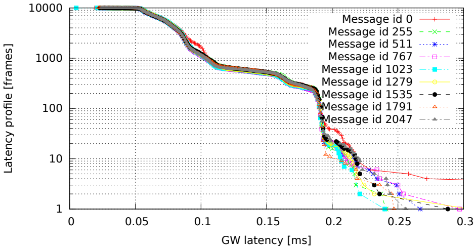
2048 GW rules (one per id, mask C00007FF), no modifications (GW kernel 3.0.4-00007-g1c8c373, Traffic 50, Load cpu)
