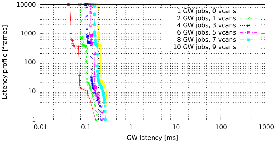
Chained GWs on multiple VCAN interfaces (GW kernel 2.6.36.2-00015-g4f1bc4e, Traffic oneatatime, Load none)
