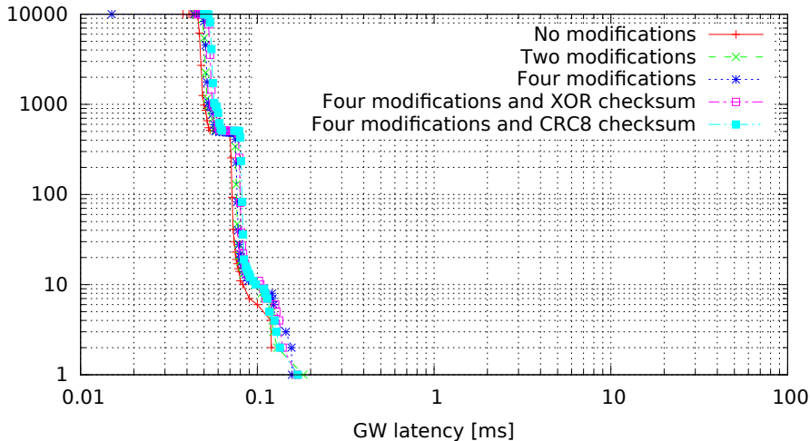
Single GW rule for all messages with modifications, 8 byte messages (GW kernel 2.6.36.2-00015-g4f1bc4e, Traffic oneatatime, Load none)
