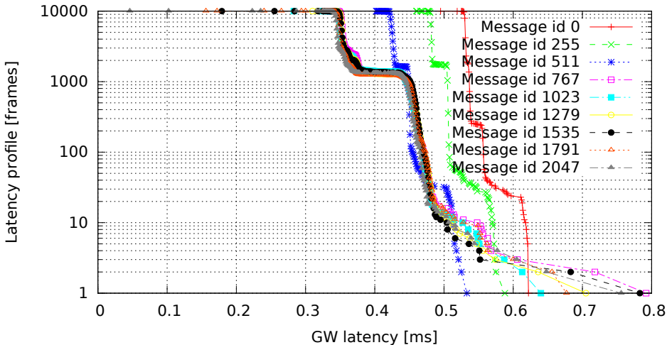
2048 GW rules (one per id, mask 0x7FF), no modifications (GW kernel 2.6.36.2-00015-g4f1bc4e, Traffic oneatatime, Load none)
